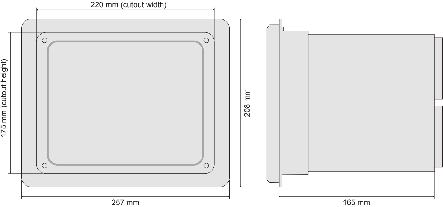
Figure 4.2 MVR-250 dimensions
