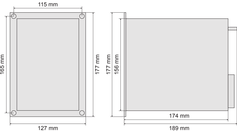
Figure 4.1 MVR-210 dimensions
